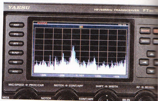
Figure 2 — Press a button and the spectrum scope goes to full-screen mode.
