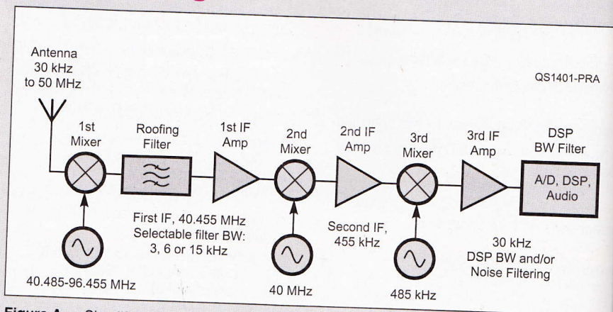
Figure A — Simplified block diagram of a modern upconverting general coverage receiver such as the FTDX1200.
