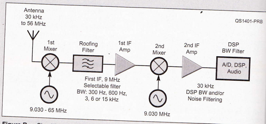
Figure B — Simplified block diagram of a modern downconverting receiver, such as the FTDX3000. Compare the narrowest bandwidth of the roofing filters in the first IF.
